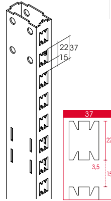
COLUMNA TROQUELADA 1 CARA COLONNE PERFORATION SIMPLE 1 CÔTÉ UPRIGHT SINGLE SLOT CHANNEL 1 SIDE TUBO PERFORAZIONE SEMPLICE 1 LATO 4814/26B 2678 mm
