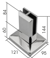
SOPORTE VIDRIO 180° INTERMEDIO support de verre intermédiaire 180° 180° intermediate glass support supporto vetro intermedio a 180°
