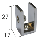
SOPORTE VIDRIO BASE PLANA PINCER VERRE BASE PLATE GLASS CLAMP FLAT BASE MORSETTO VETRO BASE PIANA 1540/032 6-10 mm
