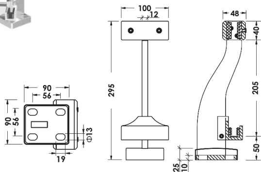
SOPORTE BARANDILLA SUPPORT GARDE-CORPS SUPPORT BALUSTRADE SUPPORTO BALAUSTRAS INOX duplex 2205
