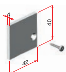
TAPA LATERAL DE CARRIL SUPERIOR COUVERTURE LATÉRALE DU RAIL SUPERIEUR TOP RAIL SIDE COVER COPERTURA LATERALE SUPERIORE *3473/001 Set dcha. izda.
