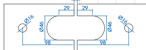
BISAGRA REGULABLE VID-VID 180° CHARNIERE REGLABLE VER-VER 180° ADJUSTABLE HINGE GLASS-GLASS 180° CERNIERA REGOLABILE VET-VET 180° *5311/R32 regulable
