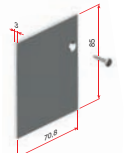
TAPA LATERAL DE CARRIL SUPERIOR COUVERTURE LATÉRALE DU RAIL SUPERIEUR TOP RAIL SIDE COVER COPERTURA LATERALE SUPERIORE *3474/001 Set dcha. izda.
