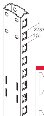
COLUMNA TROQUELADA 1 CARA COLONNE PERFORATION SIMPLE 1 CÔTÉ UPRIGHT SINGLE SLOT CHANNEL 1 SIDE TUBO PERFORAZIONE SEMPLICE 1 LATO 4814/26B 2678 mm
