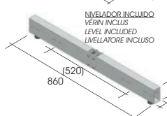
PIE AUTOPORTANTE GÓNDOLA PIED GONDOLA GONDOLA FOOT BASE GONDOLA 4818/00B
